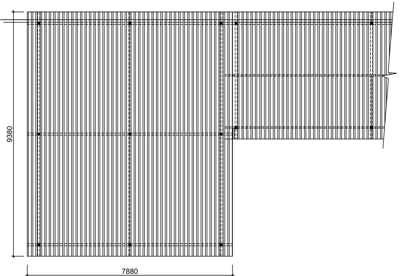
PROPOSAL TRUCK PARKING ROOFING PLAN
