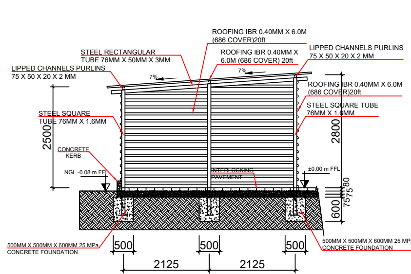
PROPOSAL WAREHOUSE. SECTION C - C
