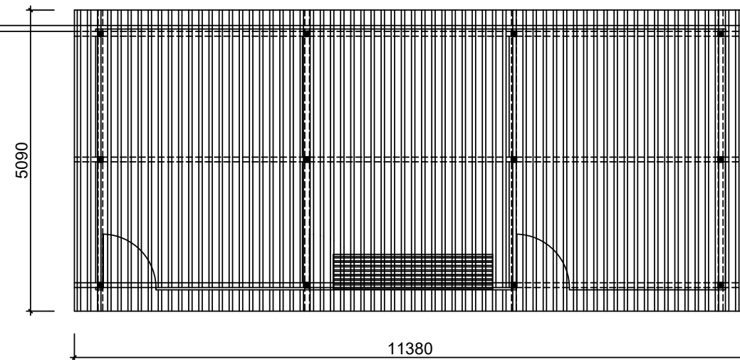
PROPOSAL WAREHOUSE ROOFING PLAN
