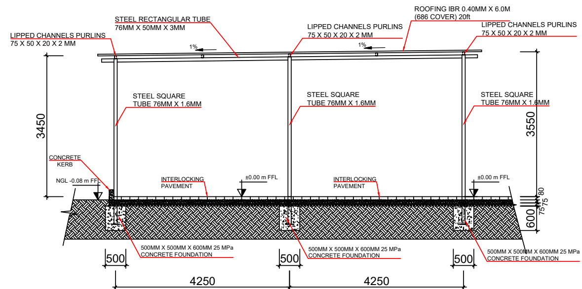
PROPOSAL TRUCK PARKING. SECTION C - C
